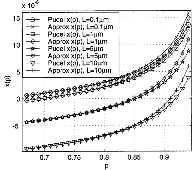
Fig. 3. Plot of x(p) from Pucel et al. model with the approximation \tilde{x}(p) as p is varied.
