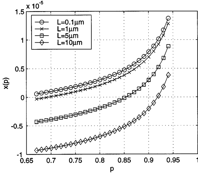
Fig. 2. Dependence of x(p) on p and L from the original Pucel et al. model.
